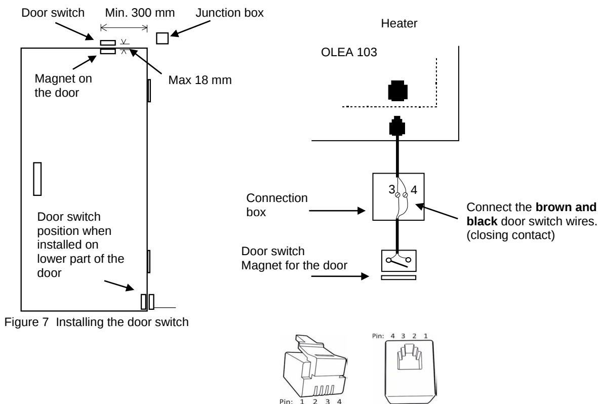
Figure 8. Pin – order of RJ 10
