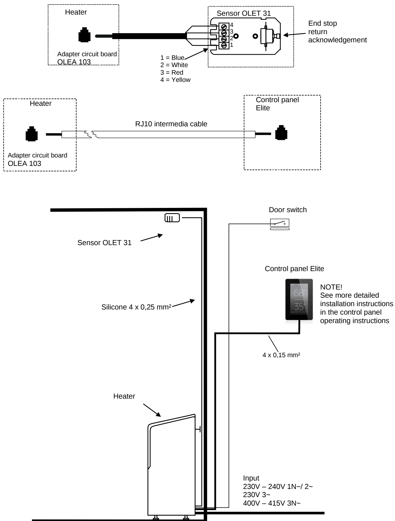
Figure 9 Principle image
