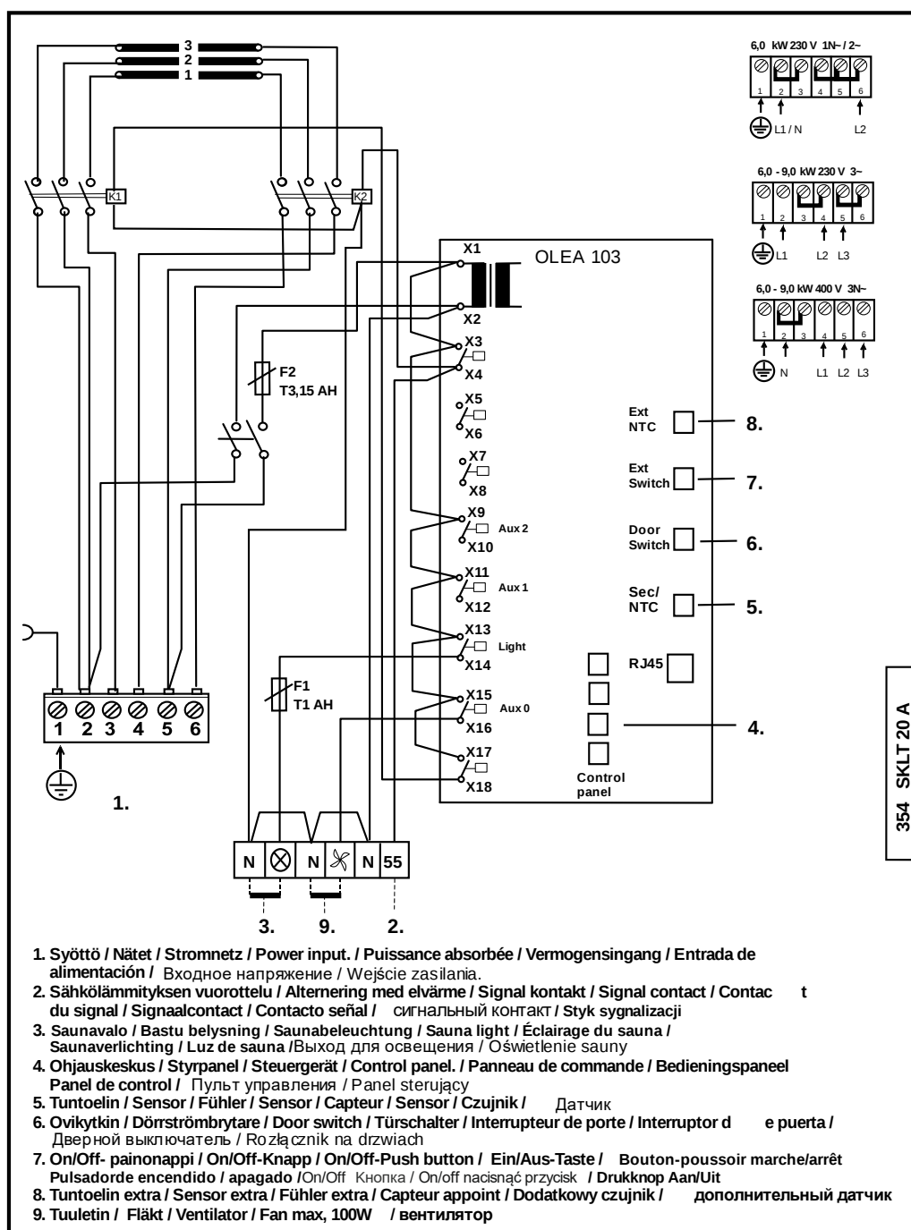
Figure 6. Schéma de raccordement
